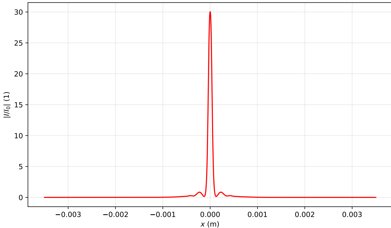
Intensity profile I(x, y = 0, z = 0.716)/I_0 , P_{in}=3.5P_{cr} , artificial time
